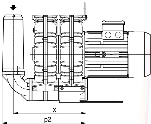
Configuration with 2 90° manifolds (Accessory)
