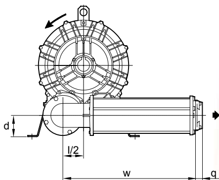
Configuration with 90° manifold and reduced dimensions
