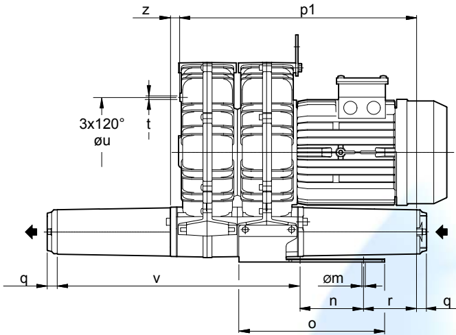
In-line silencer configuration
